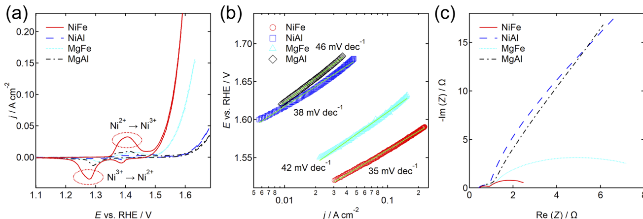
Fig. 2 (a) Cyclic voltammograms (CVs), (b) Tafel plots, and (c) Nyquist plots of NiFe-LDH/NF, NiAl-LDH/NF, MgFe-LDH/NF, and MgAl-LDH/NF in O_2 -saturated 1 \text{ mol dm}^{-3} KOH. The scans were performed at a scan rate of 5 \text{ mV}^{-1} in (a) and (b).
