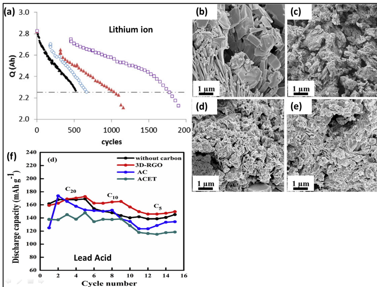
Fig. 7 (a) Cycling performance of NCR cells at different depths of discharge: 100% ( \bullet ), 75% ( \circ ), 50% ( \blacktriangle ), and 25% ( \square ) with charge at C/2 and discharge at 1C, highlighting capacity retention up to the 80% limit reproduced from ref. 11 copyright © 2015 Elsevier Ltd. (b–e) SEM images of negative active material (NAM) with various carbon additives after formation: (b) without carbon, (c) with 1.0 wt% 3D-RGO (3D Reduced Graphene Oxide) shows a more defined and structured morphology. Fig. 7d: NAM with 1.0 wt% AC (Activated Carbon) exhibits a dense and granular structure. Fig. 7e: NAM with 1.0 wt% ACET (Activated Carbon/Expanded Tubes) reveals a well-defined, fibrous morphology, enhancing conductive pathways. Fig. 7f: displays the initial discharge capacity of lead-acid test cells using different carbon additives in NAM. The graph shows a comparison of cycling performance for cells without carbon, with 3D-RGO, AC, and ACET across different charge/discharge rates (C20, C10, C5). The cells with 3D-RGO show the highest initial discharge capacity and better cycling performance compared to the others.
