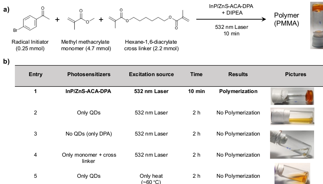
Fig. 6 Photopolymerization of MMA with InP QD-sensitized TTA-UC system. a) Schematic representation of the optimized condition for photopolymerization of MMA with InP QD-sensitized TTA-UC system. b) A table summarizing the optimized conditions for the polymerization reaction, as well as the control experiments confirming the sole involvement of the InP/ZnS QD-sensitized TTA-UC process.
