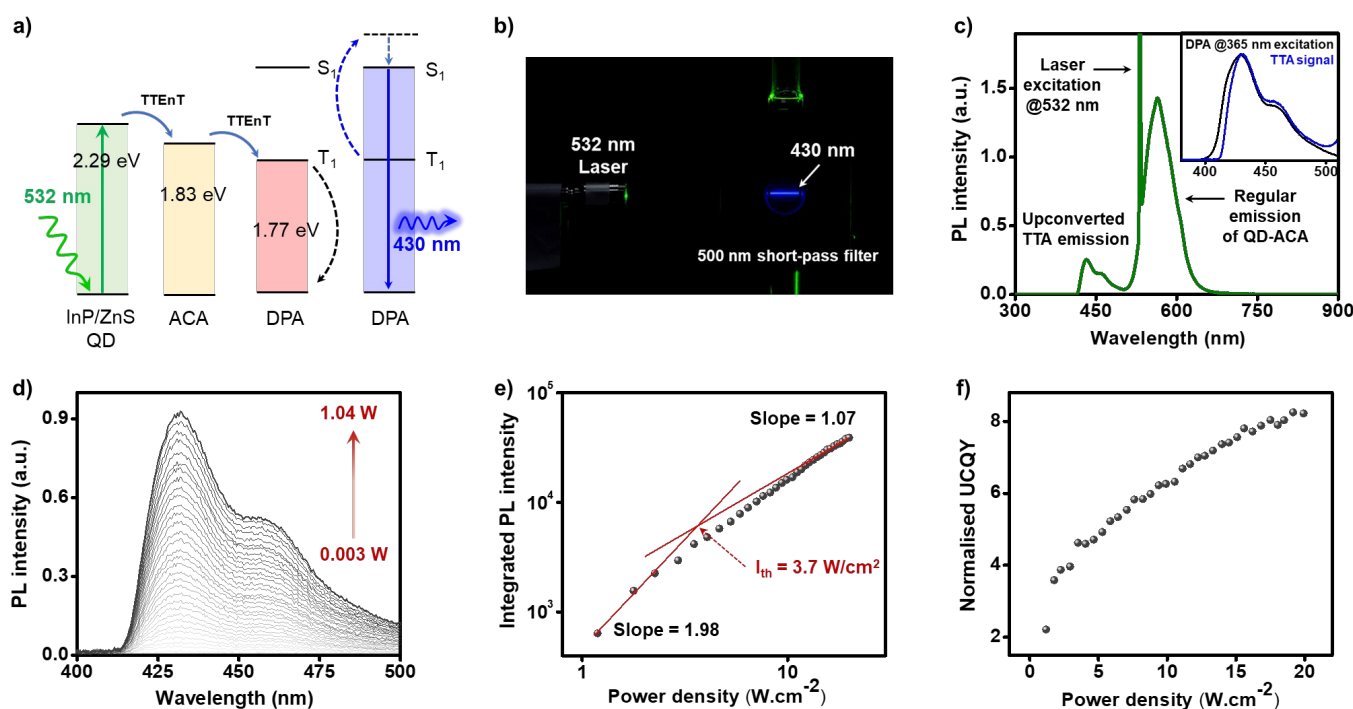
Fig. 3 InP/ZnS QD-sensitized TTA-UC system and the characterization of the TTA-UC signal. a) A schematic representation of the TTA-UC process containing InP/ZnS QD as the sensitizer, ACA as the triplet-transmitter ligand, and DPA as the annihilator. b) The optical photograph showing the bright blue upconversion signal from the cuvette (through a 500 nm short-pass filter) containing a solution of InP/ZnS-ACA and DPA, upon excitation with a 532 nm diode laser. c) The overall PL spectrum of the TTA-UC signal without any filter, showing the upconverted signal ( \lambda_{\text{max}} \sim 430 nm), the laser excitation ( \lambda_{\text{max}} \sim 532 nm), and the direct PL of the InP/ZnS QDs ( \lambda_{\text{max}} \sim 550 nm). Inset shows an overlap between the TTA-UC signal and the fluorescence of DPA (obtained by the direct excitation of DPA at \sim 365 nm), confirming that the final emission arises from DPA. The concentration of DPA was 16 mM in these studies. d) The intensity of the upconversion signal increases with increase in the power density of the laser source. e) Log-log plot of the integrated UC intensity vs laser power density showing the transition from quadratic to linear regime with I_{\text{th}} value to be 3.7 \text{ W cm}^{-2} . f) The calculated TTA-UC QY plotted as a function of the laser power density.
