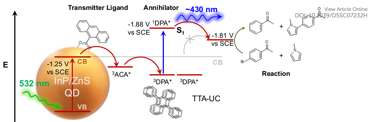
Scheme 1 Schematic representation of the TTA-UC process with ACA-capped InP/ZnS QDs as sensitizers and DPA as annihilators. The upconversion energy from the InP-based QD-sensitized TTA-UC system was used to drive the dehalogenation of substituted aryl halides, which typically require a potential exceeding the maximum achievable redox potential of InP/ZnS QDs.
