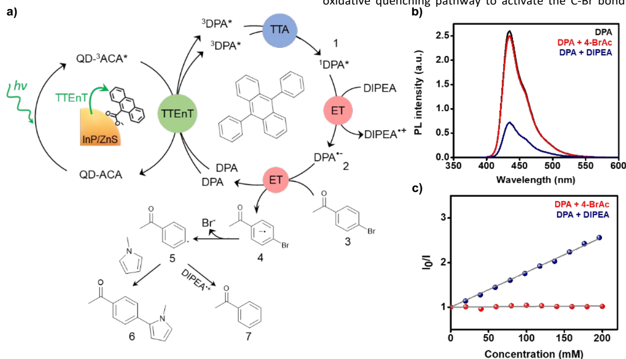
Fig. 5 a) Schematic representation of the plausible mechanism of photocatalytic redox reaction driven by the upconversion energy generated from InP/ZnS QD-sensitized TTA-UC process. ^1\text{DPA}^* formed via the TTA-UC process participates in a series of charge transfer steps, which eventually lead to the formation of the aryl radical 5 . The photophysical studies show b) a negligible quenching of the fluorescence of DPA in presence of 4-bromoacetophenone; whereas a drastic quenching of DPA fluorescence in presence of DIPEA. c) Stern-Volmer plot obtained from the relative fluorescence quenching of DPA in presence of 4-bromoacetophenone and DIPEA. This confirms that the excited ^1\text{DPA}^* first undergoes a reductive quenching in the presence of DIPEA during the photocatalytic process.
