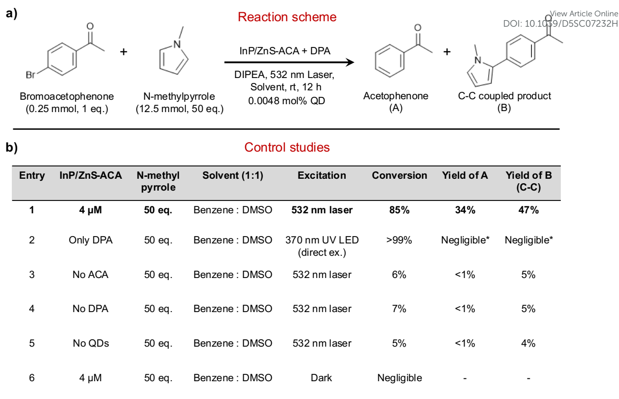
Fig. 4 Photoredox catalysis using InP/ZnS QD-sensitized TTA-UC system. a) The optimized photocatalytic redox reaction scheme for the dehalogenation of 4-bromoacetophenone and C-C coupling reaction between 4-bromoacetophenone and N-methylpyrrole. b) A table showing the optimized condition as well as other control experiments under different reaction conditions. All these experiments confirm the sole role of the TTA-UC process in enabling the photocatalytic redox reaction with visible light. (*The negligible yields obtained with direct excitation of DPA catalyst could be attributed to photodegradation due to prolonged UV irradiation)
