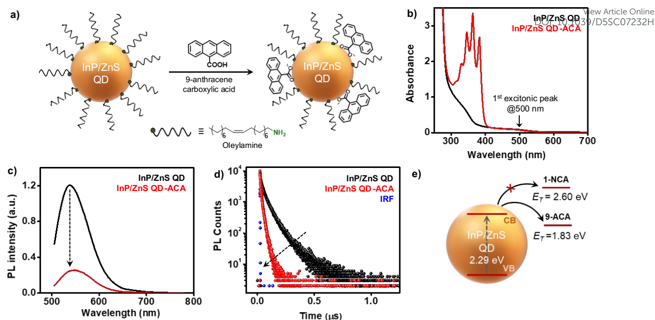
Fig. 1 a) Schematic representation of the surface functionalization of OAm-capped InP/ZnS QDs with ACA, using a ligand exchange protocol. b) Absorption spectra of InP/ZnS QDs before and after the ligand exchange with ACA, showing the characteristic absorption peaks of ACA molecules below 400 nm. The corresponding c) steady-state and d) time-resolved PL spectra of InP/ZnS QDs, showing a significant quenching after the surface functionalization with ACA molecules. e) Schematics showing the successful TTEnT from the photoexcited InP/ZnS QDs to the low-lying triplet state of the surface-bound ACA. A TTEnT from the photoexcited InP/ZnS QDs to the triplet state of NCA is thermodynamically not feasible, which was observed in the experiment as well (Fig. S3†).
