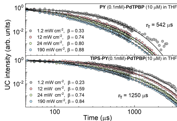
Fig. 5 Normalized UC transients of PY and TIPS-PY on a log–log scale at different excitation densities (indicated) upon sensitization with PdTPBP at 640 nm. Circles present experimental data, while solid lines show global fits with a shared \tau_{\text{T}} .
