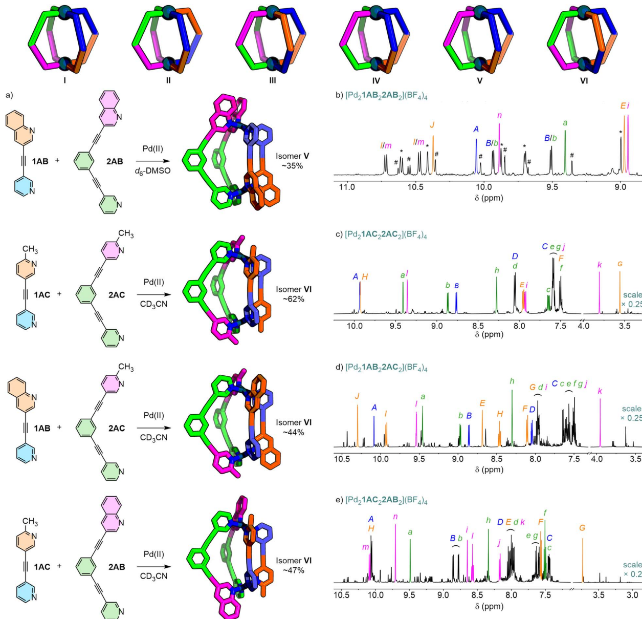
Fig. 8 (a) The selective formation of particular isomers of Pd 2 L A 2 L B 2 -type cages (GXN2-xTB geometry-optimised models shown) from combinations of ligands 1AB/1AC and 2AB/2AC was observed. Partial 1 H NMR spectra (600 MHz, 298 K) of (b) [Pd 2 1AB 2 2AB 2 ](BF 4 ) 4 (d 6 -DMSO) with peaks assigned to major isomer V labelled (# = minor isomer; * = [Pd 2 2AB 4 ] 4+ ); and (c) [Pd 2 1AC 2 2AC 2 ](BF 4 ) 4 , (d) [Pd 2 1AB 2 2AC 2 ](BF 4 ) 4 , and (e) [Pd 2 1AC 2 2AB 2 ](BF 4 ) 4 (all CD 3 CN) with peaks assigned to major product, isomer VI , labelled.
