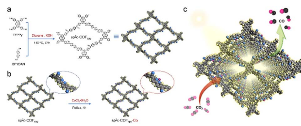
Fig. 5 (a) Synthesis of sp 2 c-COFdpy and (b) sp 2 c-COFdpy-Co. (c) Schematic CO 2 photoreduction on the as-prepared sp 2 c-COFdpy-Co. Reproduced from ref. 40 with permission from Elsevier, copyright 2020.
