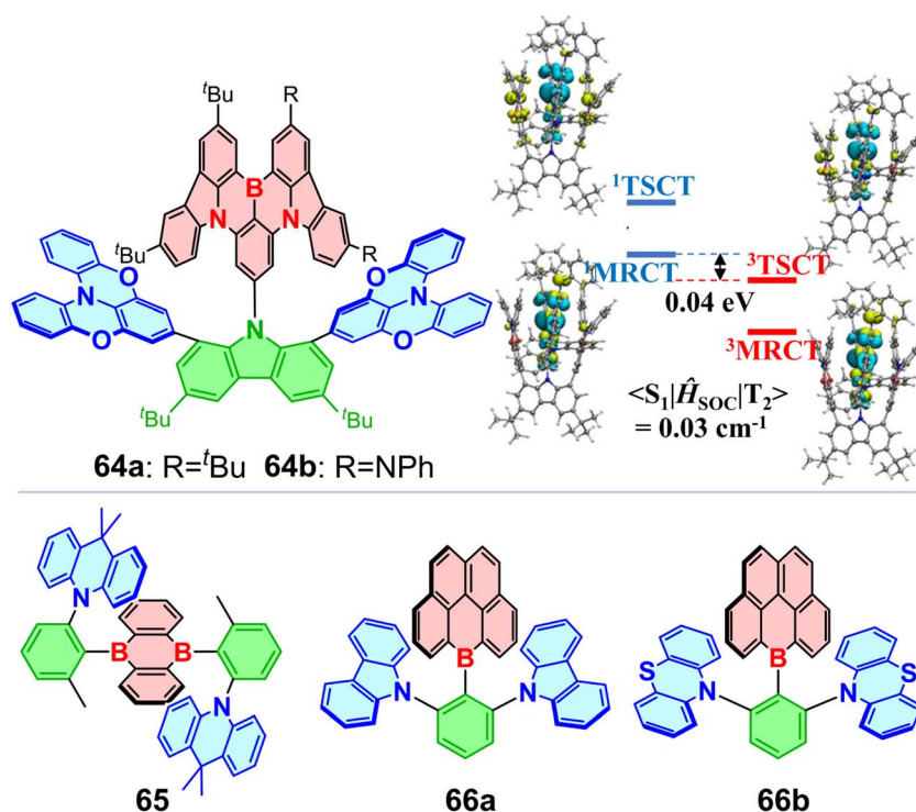
Fig. 20 TSCT OBCTs with different planar boron acceptors. The illustration showing calculated hole (green) and electron (blue) distributions and energy gaps of the 1,3 MRCT and 1,3 TSCT excited states for 64b . Copyright 2023, John Wiley & Sons.
