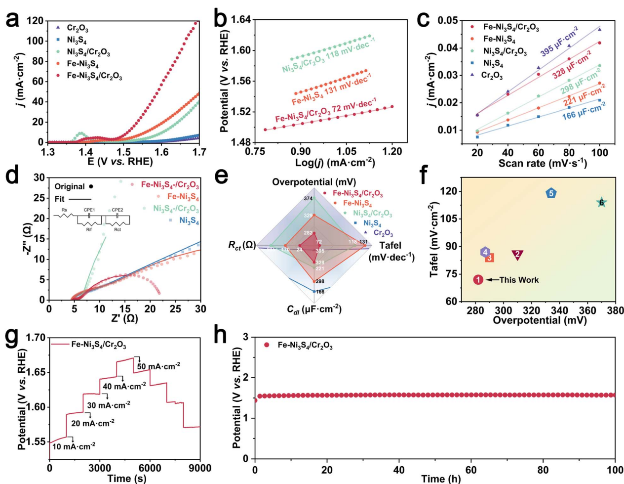
Fig. 3 OER activity in 1 M KOH solution. (a) LSV polarization curves, (b) Tafel plots, (c) C_{dl} values, and (d) Nyquist plots at 1.5 V versus RHE of Ni 3 S 4 , Ni 3 S 4 /Cr 2 O 3 , Fe-Ni 3 S 4 , and Fe-Ni 3 S 4 /Cr 2 O 3 . (e) Radar chart for comparison of comprehensive catalytic performance. (f) A comparison with other recently reported catalysts. (g) CP curve of Fe-Ni 3 S 4 /Cr 2 O 3 at different current densities. (h) CP curve of Fe-Ni 3 S 4 /Cr 2 O 3 at 10 mA cm -2 .
