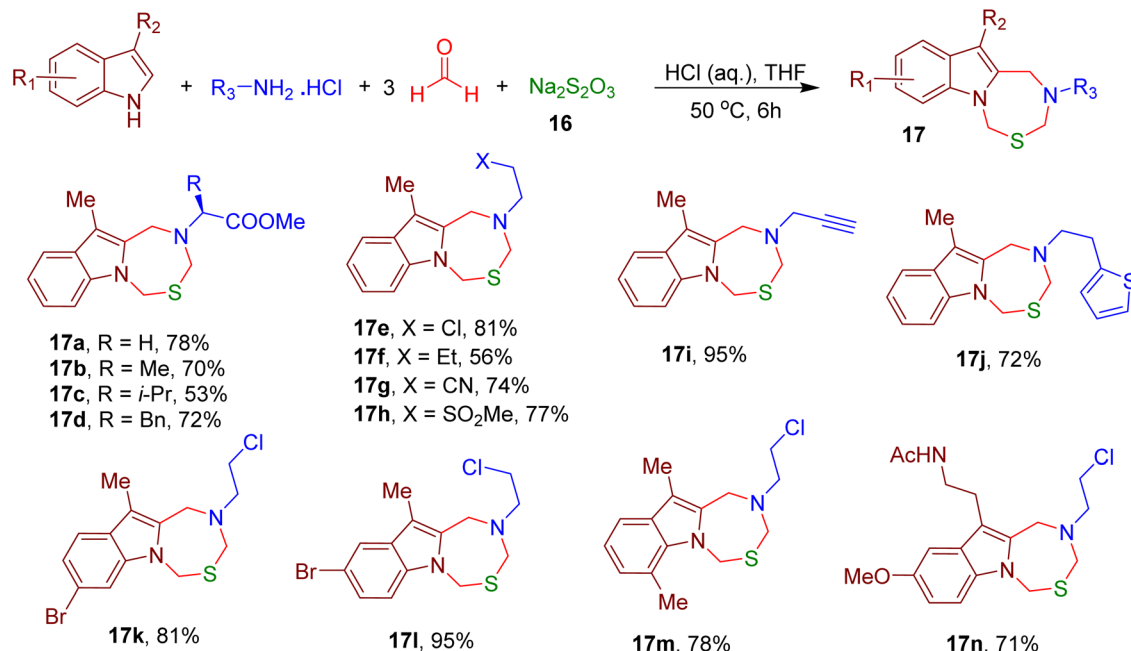
Fig. 9 MCR for the synthesis of indole-fused thiazepines.
