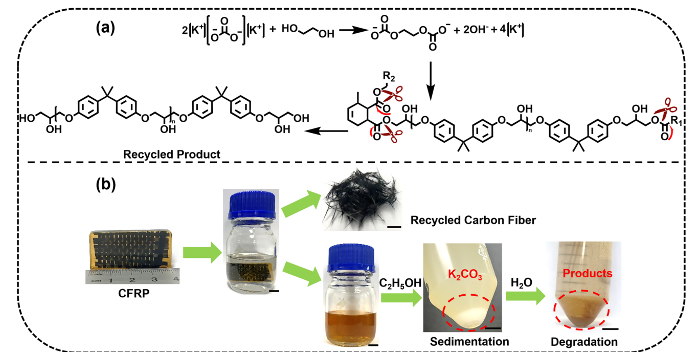
Fig. 5 (a) Schematic diagram of ester bond cleavage and (b) nondestructive recovery of carbon fibers from the composite materials. Scale bars: 1 cm.
