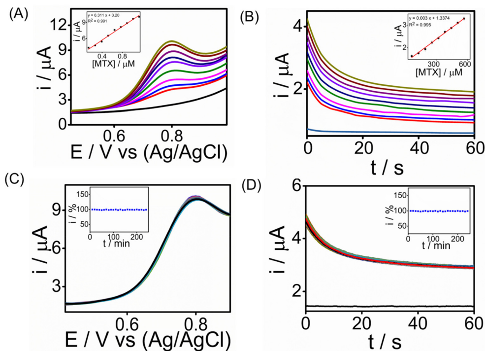
Fig. 6 Electroanalytical performance of the SPCE/PrGO-PPy-Au sensor in serum. (A) SWV analysis of MTX in serum (pH 7.4) conducted over a concentration range of 130 nM–1 \mu M. (B) Chronoamperometric measurements of MTX in serum (pH 7.4) recorded for a concentration range of 65 nM–565 nM. (C) Stability studies of MTX with a concentration of 1.3 \mu M in serum (pH 7.4) conducted for 4 hours with measurements taken every 10 minutes. (D) Stability studies of MTX with a concentration of 1.3 \mu M in serum (pH 7.4) for 4 hours with readings taken every 10 minutes. (The corresponding calibration curves are displayed in all the inset graphs.)
