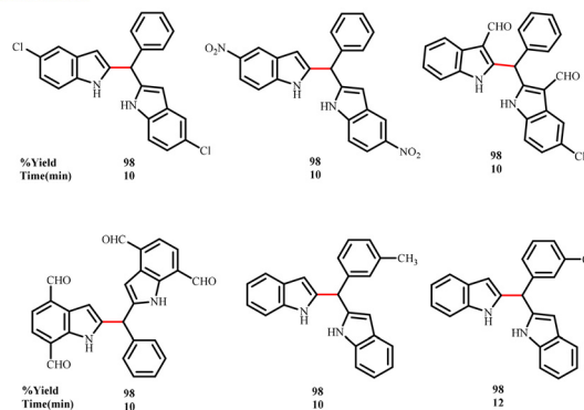
Scheme 36 Bis(indolyl)methane synthesis in the presence of \text{Fe}_3\text{O}_4@\text{MgCuAl-LDH}@\text{CS}/\text{Cu(II)} (Rashtiani et al. ).
