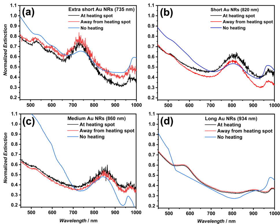
Fig. 6 Extinction spectra of Au NR/hydrogels under localized heating with 785 nm laser excitation for 15 min. (a) Extra short Au NRs with LSPR at 735 nm, (b) short Au NRs with LSPR at 820 nm, (c) medium Au NRs with LSPR at 860 nm, and (d) long Au NRs with LSPR at 934 nm. Spectra were recorded under three conditions: no heating (blue), at the heating spot (black), and away from the heating spot (red). The LSPR and TSPR peaks remain unchanged across all heating conditions, demonstrating the thermal stability of the nanorods embedded in the hydrogel matrix.
