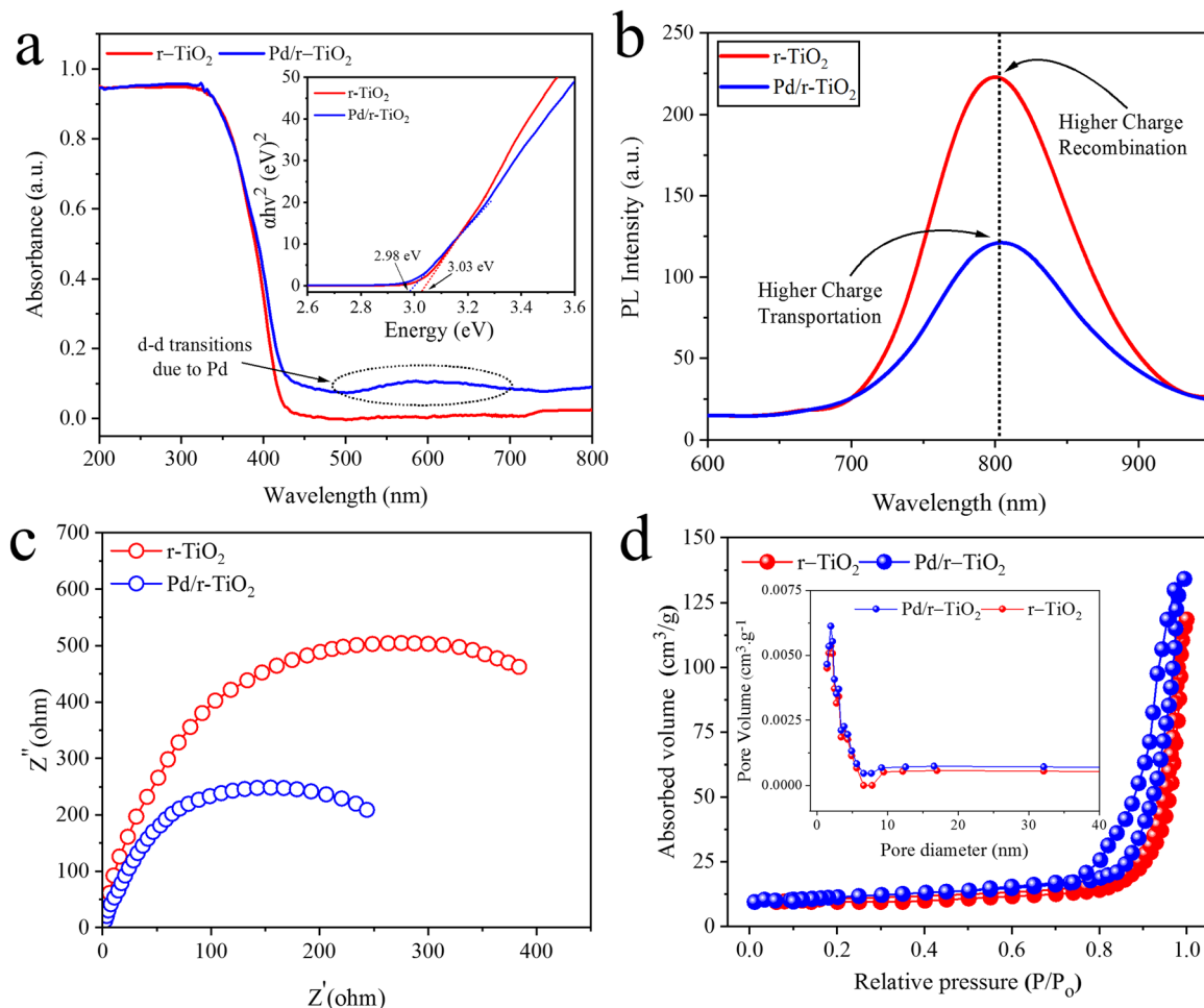
Fig. 5 (a) UV-Vis/DRS results, inset: band gap energy diagrams, (b) PL results, (c) EIS analysis, and (d) BET analysis, inset: pore volume/size distribution of r\text{-TiO}_2 and \text{Pd}/r\text{-TiO}_2 .
