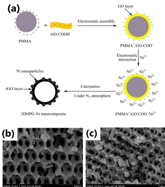
Fig. 9 (a) Schematic illustrating the synthesis for three-dimensional porous hierarchical graphene. (b and c) SEM images of three-dimensional porous hierarchical graphene. This figure has been reproduced from ref. 213 with permission from Elsevier, copyright 2018.
