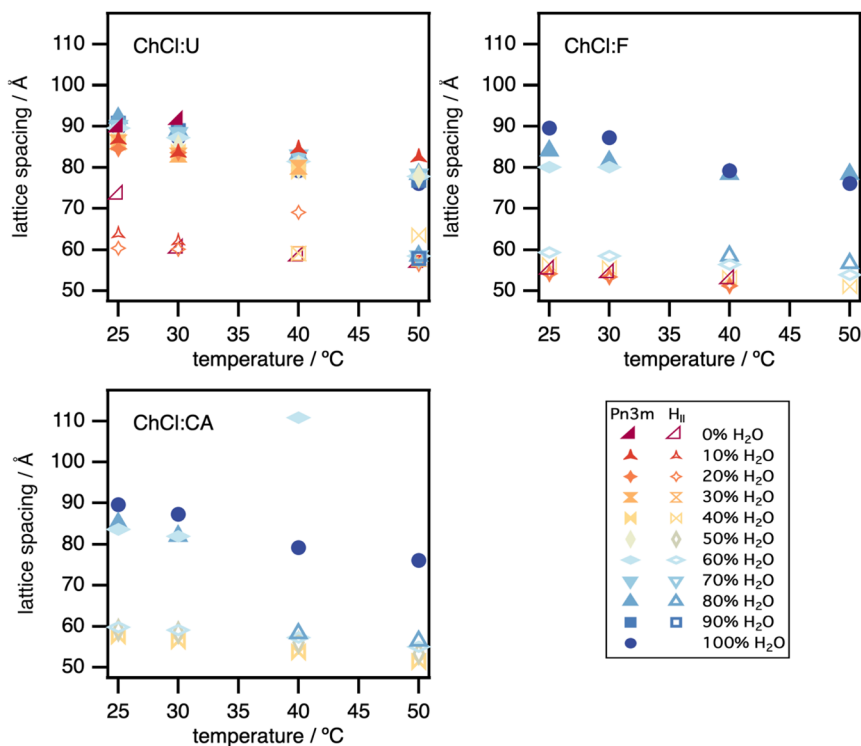
Fig. 7 Lattice spacings for the Pn3m cubic and H_{II} phases observed for monoolein in ChCl : U-water, ChCl : F-water and ChCl : CA-water mixtures. The error bars are smaller than the marker sizes. Where two H_{II} phases are observed, the larger lattice spacing is plotted.
