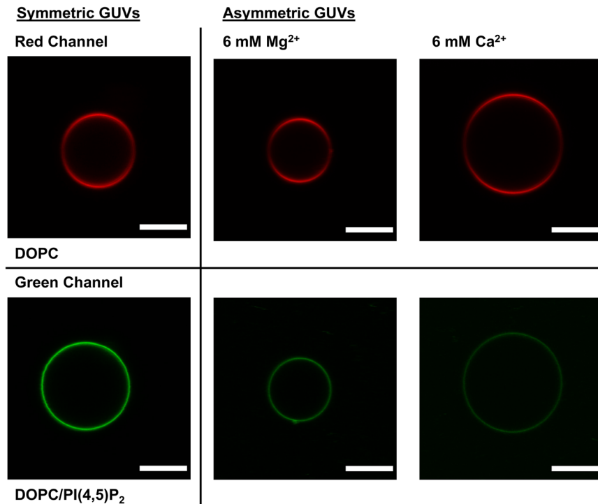
Fig. 2 Images of symmetric control GUVs (left column) and asymmetric GUVs (right column) prepared with either 6 mM Mg^{2+} or 6 mM Ca^{2+} as indicated. Scale bar = 10 \mu m. sGUV controls were prepared in 100 mM sucrose but were imaged in 100 mM glucose for a total buffer composition of 100 mM saccharide, 97 mM NaCl, 50 mM KCl, 1 mM Na_2 -EDTA, 20 mM HEPES, pH = 7.4 on either side of the vesicle bilayer. aGUVs were imaged above the SLB after hemifusion in the resuspension buffer plus the indicated amount of bivalent cation and \sim 7 mM Na_2 EDTA. Vesicles prepared with DiD' appear dimmer at the equator due to a well-known polarization artifact arising from the properties of the fluorophore and are not due to phase separation in a pure DOPC bilayer.
