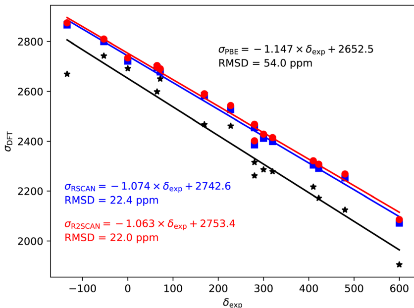
Fig. 5 ^{79/81}\text{Br} magnetic shieldings, \sigma , calculated with the PBE (black), rSCAN (blue) and \text{r}^2\text{SCAN} (red) functionals vs. experimental chemical shifts, \delta . For each functional the line of best fit is given.
