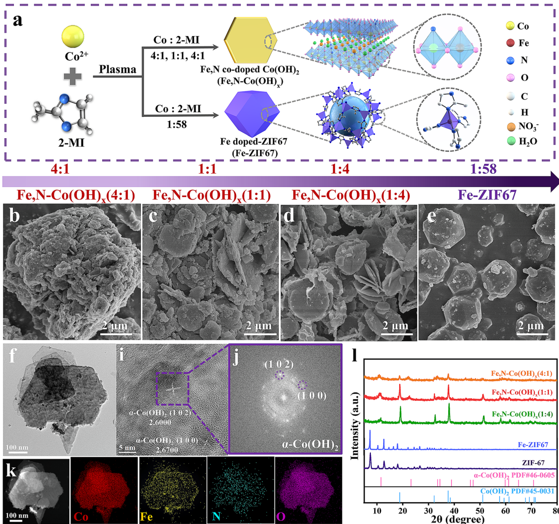
Fig. 1 Preparation process and morphology of electrocatalysts. (a) Schematic of the synthesis of Fe,N co-doped \text{Co(OH)}_2 (i.e., \text{Fe}_x\text{N-Co(OH)}_x ) and Fe-doped ZIF67 (i.e., \text{Fe-ZIF67} ) induced by plasma in water. (b)–(e) SEM images of (b) \text{Fe}_x\text{N-Co(OH)}_x (4:1), (c) \text{Fe}_x\text{N-Co(OH)}_x (1:1), (d) \text{Fe}_x\text{N-Co(OH)}_x (1:4), and (e) Fe-ZIF67. (f)–(k) Morphology and elemental distribution of \text{Fe}_x\text{N-Co(OH)}_x (1:1): (f) TEM images, (i) HAADF-STEM images, (j) corresponding FFT pattern, and (k) EDS mapping images. (l) XRD patterns of \text{Fe}_x\text{N-Co(OH)}_x (4:1) (orange line), \text{Fe}_x\text{N-Co(OH)}_x (1:1) (red line), \text{Fe}_x\text{N-Co(OH)}_x (1:4) (green line), and Fe-ZIF67 (purple line).
