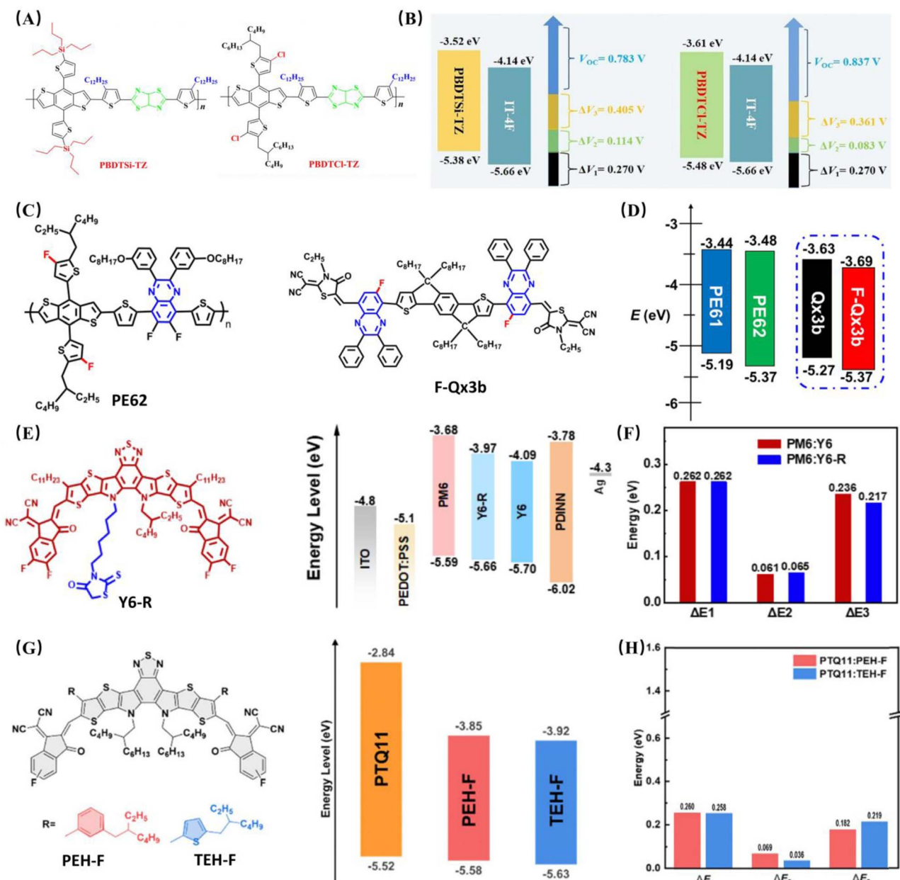
Fig. 5 (A) Chemical structures of PBDSi-TZ and PBDCI-TZ; (B) energy loss of devices based on PBDSi-TZ:IT-4F and PBDCI-TZ:IT-4F. 86 Copyright 2020 WILEY-VCH. (C) Chemical structures of PE62 and F-Qx3b; (D) energy levels of PE62 and F-Qx3b. 87 Copyright 2021 Elsevier. (E) Chemical structure of Y6-R and energy level of its device; (F) energy loss of devices based on PM6:Y6 and PM6:Y6-R. 91 Copyright 2025 American Chemical Society. (G) Chemical structures and energy levels of PEH-F and TEH-F; (H) energy loss of devices based on PTQ11:PEH-F and PTQ11:TEH-F. 92 Copyright 2025 Royal Society of Chemistry.
