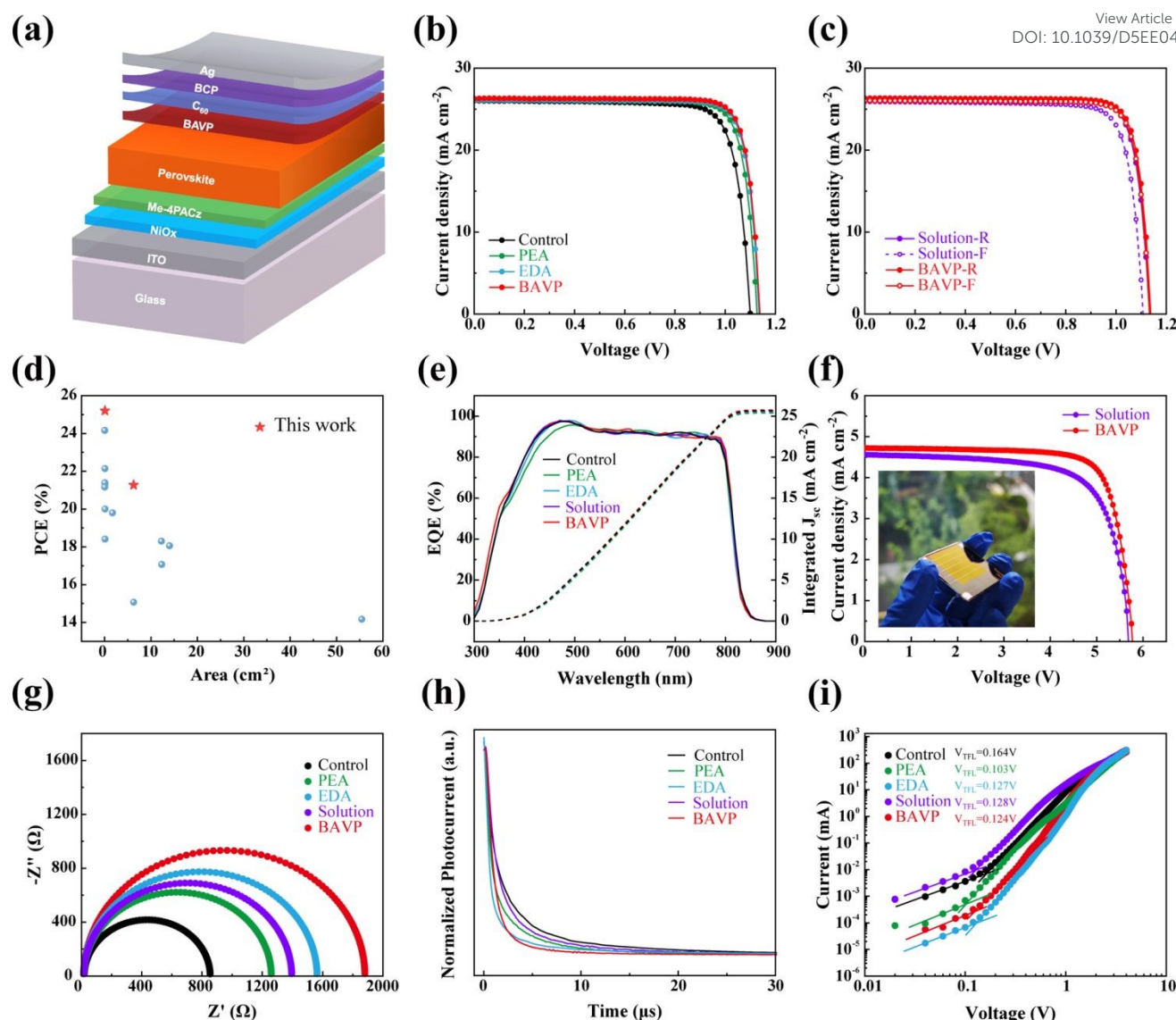
Figure 4. (a) Device structure of the inverted PSCs used in this work. The J - V curves of the best small area devices (b) without and with different amine vapor treatments and (c) with solution-based or vapor-based passivation methods using PEA/EDA mixed amines. (d) Representative PCEs of inverted FAPbI 3 -based PSCs and PSMs fabricated by blade-coating methods. (e) EQE spectra of the small area devices without and with different passivation methods using different amines. (f) The J - V curves and images of PSMs with different passivation methods. (g) The electrochemical impedance spectroscopy and (h) transient photocurrent of the devices without and with different amine vapor treatments. (i) SCLC characteristics of the electron-only devices without and with different amine vapor treatments.
