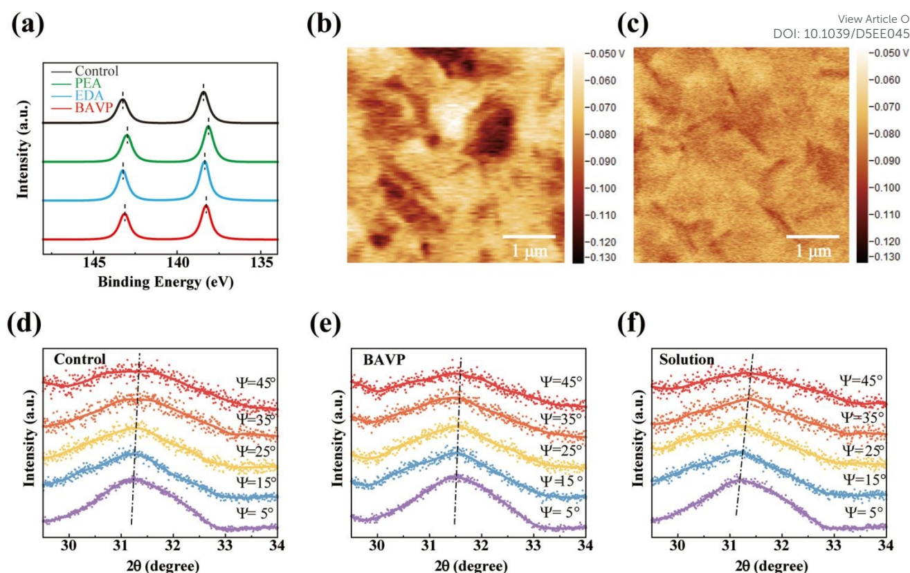
Figure 2. (a) XPS spectra of Pb 4f for the control, PEA vapor, EDA vapor and BAVP treated perovskite films. KPFM images of (b) solution passivated and (c) BAVP treated FAPbI 3 perovskite films. Depth-resolved GIXRD spectra of (d) the control, (e) BAVP and (f) solution passivated FAPbI 3 perovskite films at different \Psi angles (from 5° to 45°).
