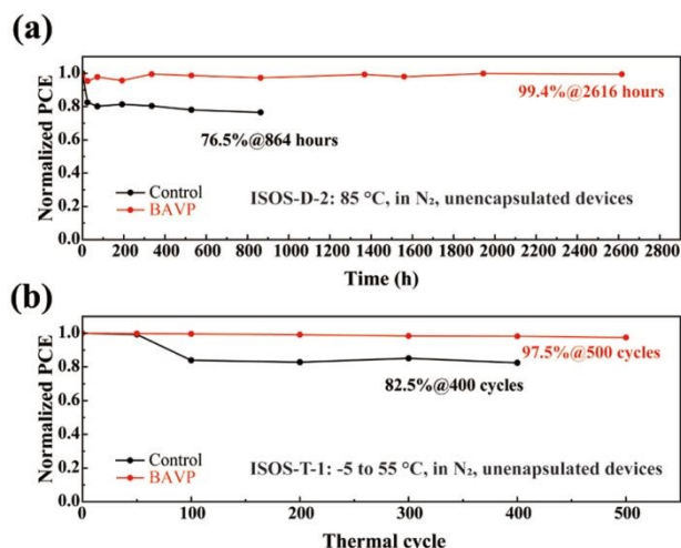
Figure 5. (a) Thermal stability test of the unencapsulated PSCs under 85 °C in N 2 following the ISOS-D-2 protocol. (b) Thermal-cycling stability test of the unencapsulated PSCs under a temperature range of -5 to 55 °C in N 2 following the ISOS-T-1 protocol.
