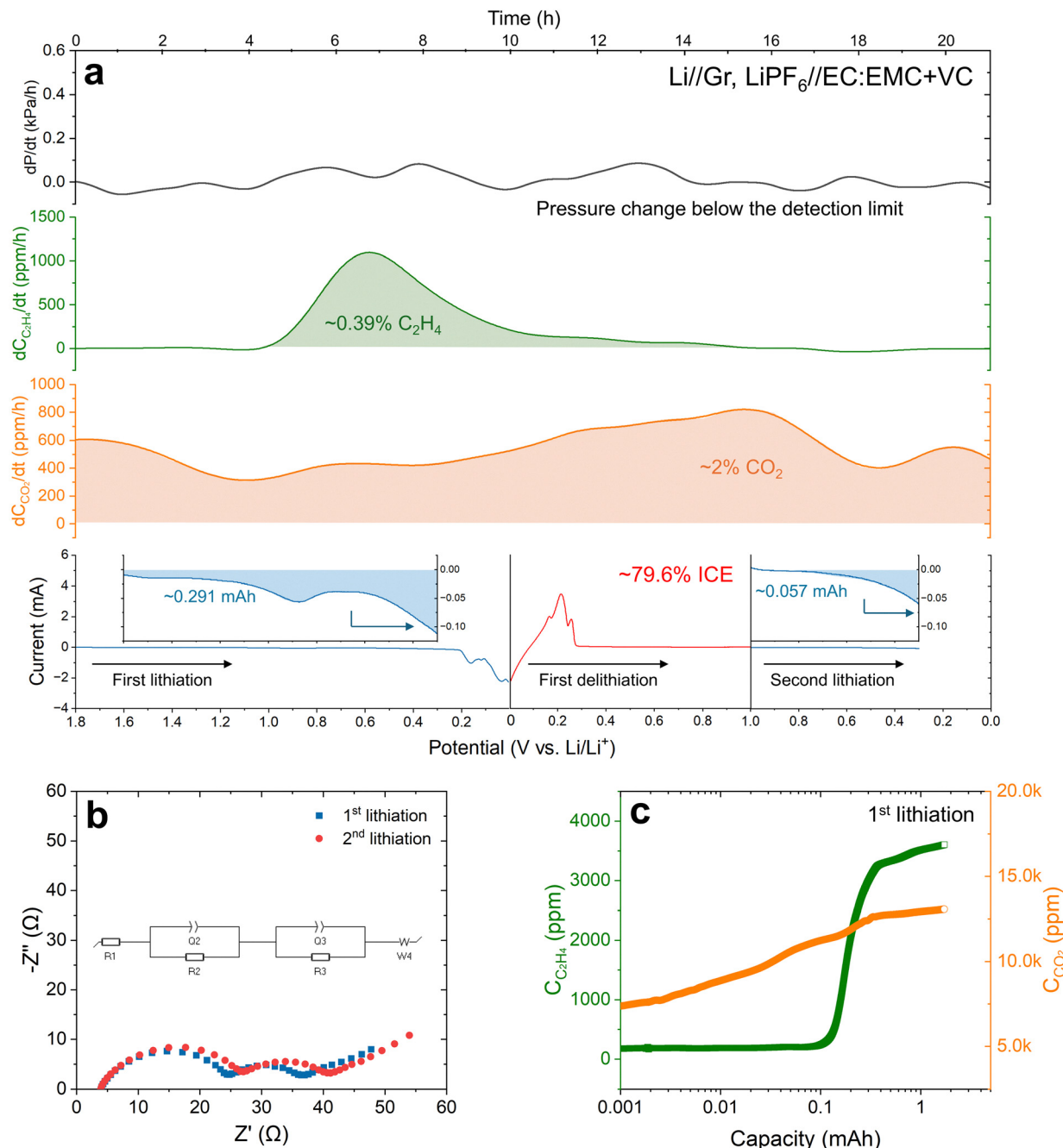
Fig. 7 Operando monitoring of gas evolution in the Li-graphite half-cell that undergoes cyclic voltammetry at a scan rate of 0.05 \text{ mV s}^{-1} with 1 \text{ M LiPF}_6 in EC:EMC:VC (3:7 vol% + 2 vol% VC) as the electrolyte. (a) The obtained CV curves are plotted in conjunction with the change in concentrations of \text{C}_2\text{H}_4 , \text{CO}_2 , and in overall gas pressure. The detailed current variation from 1.8 V to 0.3 V vs. \text{Li/Li}^+ of the first lithiation and from 1 V to 0.3 V vs. \text{Li/Li}^+ of the second lithiation is provided in the insets by zooming in the y-axis. The blue shading of the first lithiation represents the electric charge consumed for the SEI formation and associated gas evolution. (b) The EIS spectra obtained after the initial and the second cathodic scan. (c) Evolution of \text{C}_2\text{H}_4 and \text{CO}_2 concentrations during the initial lithiation of graphite.
