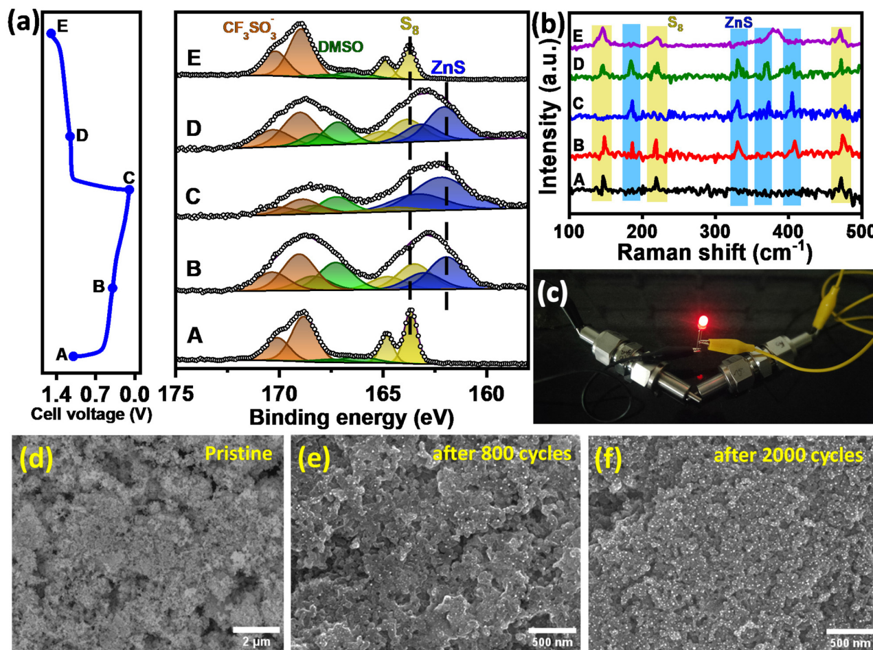
Fig. 5 (a) XPS and (b) Raman spectra of S@AC at different charge–discharge voltages; (c) photograph of an LED powered by assembling two Zn||Zn batteries using the AZ/DMSO/ZnI 2 electrolyte; FESEM images of the sulfur cathode: (d) pristine, (e) after 800 cycles, and (f) after 2000 cycles.
