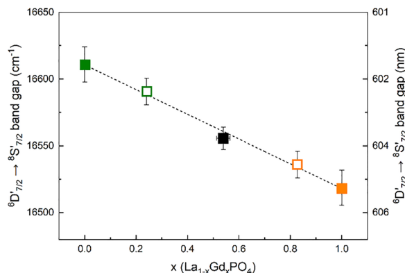
Fig. 7 Cm III excitation peak maxima (band gap energy) as a function of Gd III substitution ( x ) in La 1-x Gd x PO 4 monazite solid solutions. Adapted with permission from ref. 51. Copyright 2018 American Chemical Society.
