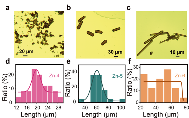
Fig. 3 Optical micrographs and length distributions of single crystals of (a and d) Zn-4 , (b and e) Zn-5 , and (c and f) Zn-6 . Lengths were measured for 25 single crystals randomly selected from each sample.
