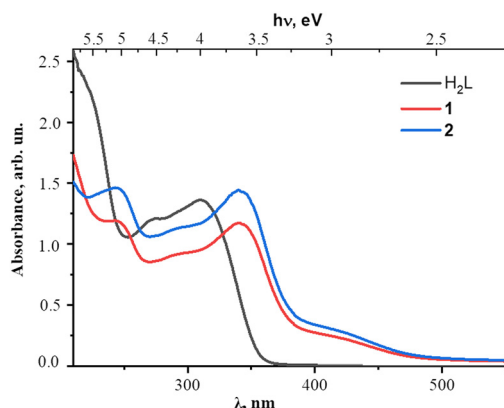
Fig. 5 Absorption spectra of the \text{H}_2\text{L} ligand and \text{Fe}(\text{III}) coordination compounds 1 and 2 .
