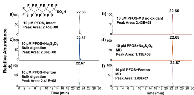
Fig. 3 EIC of the signal [PFOS-H]^- of 10 \mu\text{M} PFOS (a) before degradation, (b) after degradation in microdroplets without oxidant additive, (c) after degradation in bulk solution using \text{S}_2\text{O}_8^{2-} additive, (d) after degradation in microdroplets containing \text{S}_2\text{O}_8^{2-} , (e) after degradation in bulk solution using Fenton's reagent additive, and (f) after degradation in microdroplets containing Fenton's reagent.
