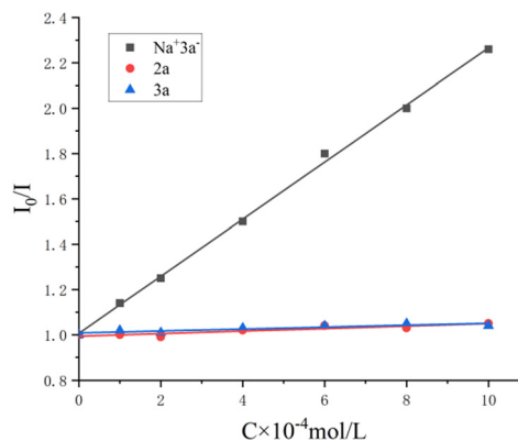
Fig. 1 Stern–Volmer plots. I_0 is the inherent fluorescence intensity of [Ir(dtbbpy)(ppy) 2 ]PF 6 . I is the fluorescence intensity of [Ir(dtbbpy)(ppy) 2 ]PF 6 in the presence of \text{Na}^+3a^- , 2a or 3a .
