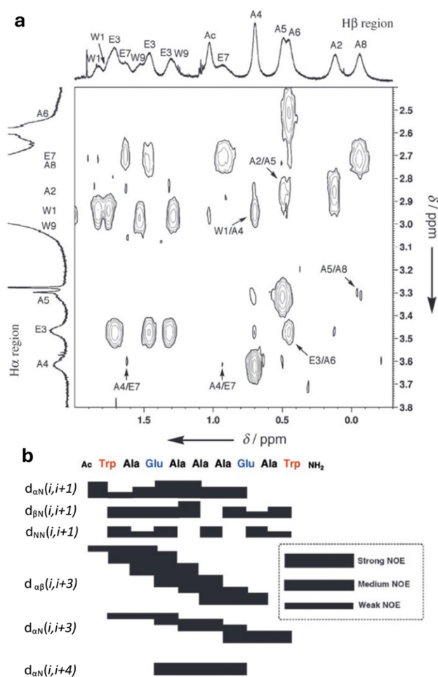
Fig. 3 (a) Selected NOESY spectrum for the assignment of bound peptide (600 MHz, \text{H}_2\text{O}/\text{D}_2\text{O} = 9/1 , 27 °C, 100 mM phosphate buffer, pH 6.8), [\text{Z}] = 10 mM, [\text{peptide}] = 2.5 mM. Proton resonances labelled with single letter amino acid code and residue number corresponding to peptide in Fig. 2a; (b) NOE correlations for peptide 2 . Reproduced with permission from ref. 16.
