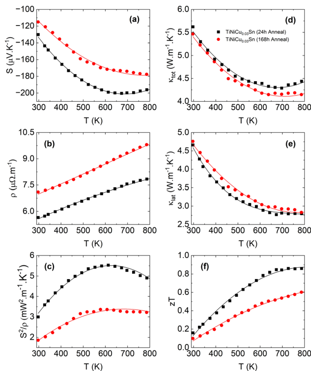
Fig. 2 Temperature dependent thermoelectric properties for the 24 h and 168 h annealed \text{TiNiCu}_{0.03}\text{Sn} samples. Panel (a) shows the Seebeck coefficient S , (b) the electrical resistivity \rho , (c) the power factor S^2/\rho , (d) the total thermal conductivity \kappa , (e) the lattice thermal conductivity \kappa_{\text{L}} , and (f) the figure of merit zT . Lines are guides to the eye.
