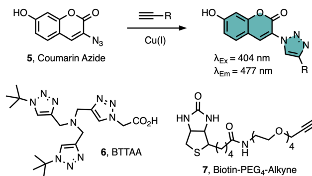
Scheme 1 Schematic of the fluorogenic assay to monitor product formation under different CuAAC conditions. Also shown are the structures of the Cu I -stabilizing ligand BTAA ( 6 ) and biotin-PEG 4 -alkyne ( 7 ).
