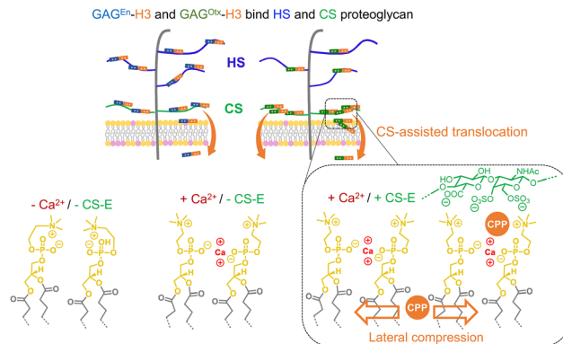
Fig. 8 Schematic representation of the proposed role of GAGs in the internalization mechanism of the chimeric peptides studied herein: GAG Otx and GAG En , H3 and chimeric GAG Otx -H3 and GAG En -H3. CS are located at the vicinity of the lipid bilayer while HS are more distal. The chimeric CPPs bind to HS- and CS- proteoglycans (CS-E bind PC lipids in the presence of \text{Ca}^{2+} , leading to an overall anionic complex). Therefore, there are no longer repulsion forces between the cationic choline head-group and the cationic peptide, could then insert deeper into the lipid bilayer to cross it.
