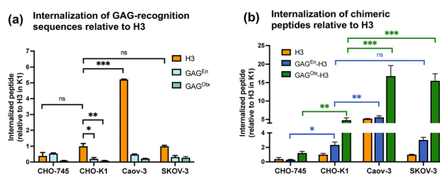
Fig. 2 Quantity of (a) H3 and GAG-binding sequences and (b) chimeric peptides internalized in one million cells after 1 hour incubation with peptides (7 μM) at 37 °C, determined by MALDI-TOF MS. 25,26 The amounts were normalized relative to H3 internalization in K1 cells.
