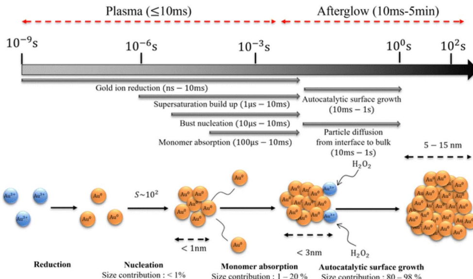
Fig. 3 Schematic of the formation mechanism of gold nanoparticles in a plasma–droplet system. 48
