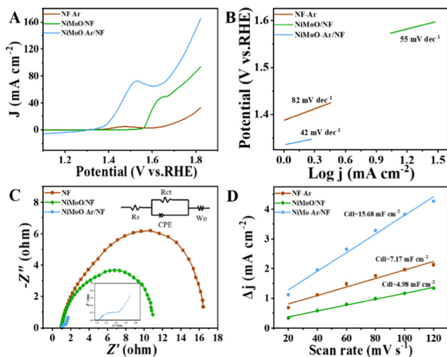
Fig. 4 (A) Polarization curve comparison of NF-Ar, NiMoO/NF, and NiMoO-Ar/NF in electrolyte containing 15 mM BA. (B) Tafel curves corresponding to figure A. (C) Comparison of the impedance of NF-Ar, NiMoO/NF and NiMoO-Ar/NF in electrolyte containing 15 mM BA. (D) C_{dl} curves of NF-Ar, NiMoO/NF and NiMoO-Ar/NF in an electrolyte containing 15 mM BA.
