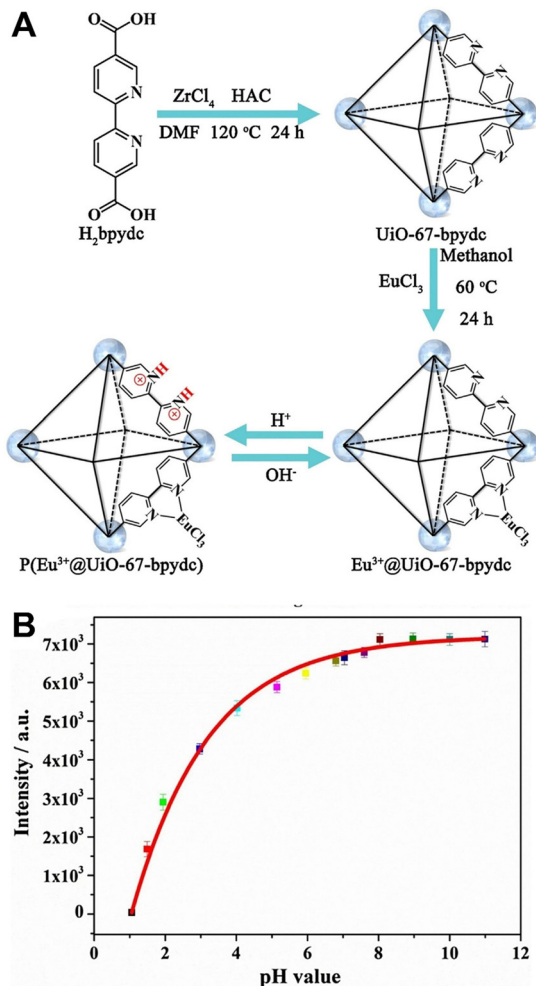
Fig. 4 (A) Protonation and deprotonation of \text{Eu}@UiO-67\text{-bpydc} . (B) The relationship between the emission intensity at 615 nm and the pH value. Reproduced with permission from ref. 42 Copyright: 2018, Elsevier.
