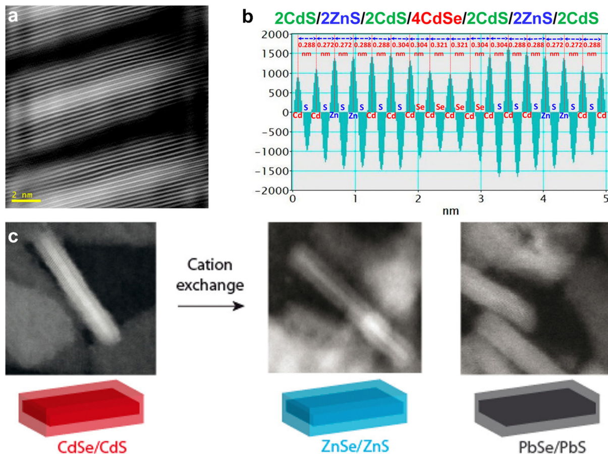
Fig. 11 (a) HAADF-STEM image of 2CdS/2ZnS/2CdS/4CdSe/2CdS/2ZnS/2CdS formed by c-ALD using Li 2 S/Li 2 Se and anhydrous Cd(HCOO) 2 /Zn(OAc) 2 powders as the sources of chalcogen and metal precursors, respectively; (b) the interplanar distances for this structure shown in (a); (c) schematic representation of the cation exchange of CdSe/CdS core/shell NPLs to ZnSe/ZnS and PbSe/PbS NPLs with corresponding HAADF-STEM images. Panels (a) and (b) are adapted with permission from The American Chemical Society. 240 Panel (c) is adapted with permission from The American Chemical Society. 254
