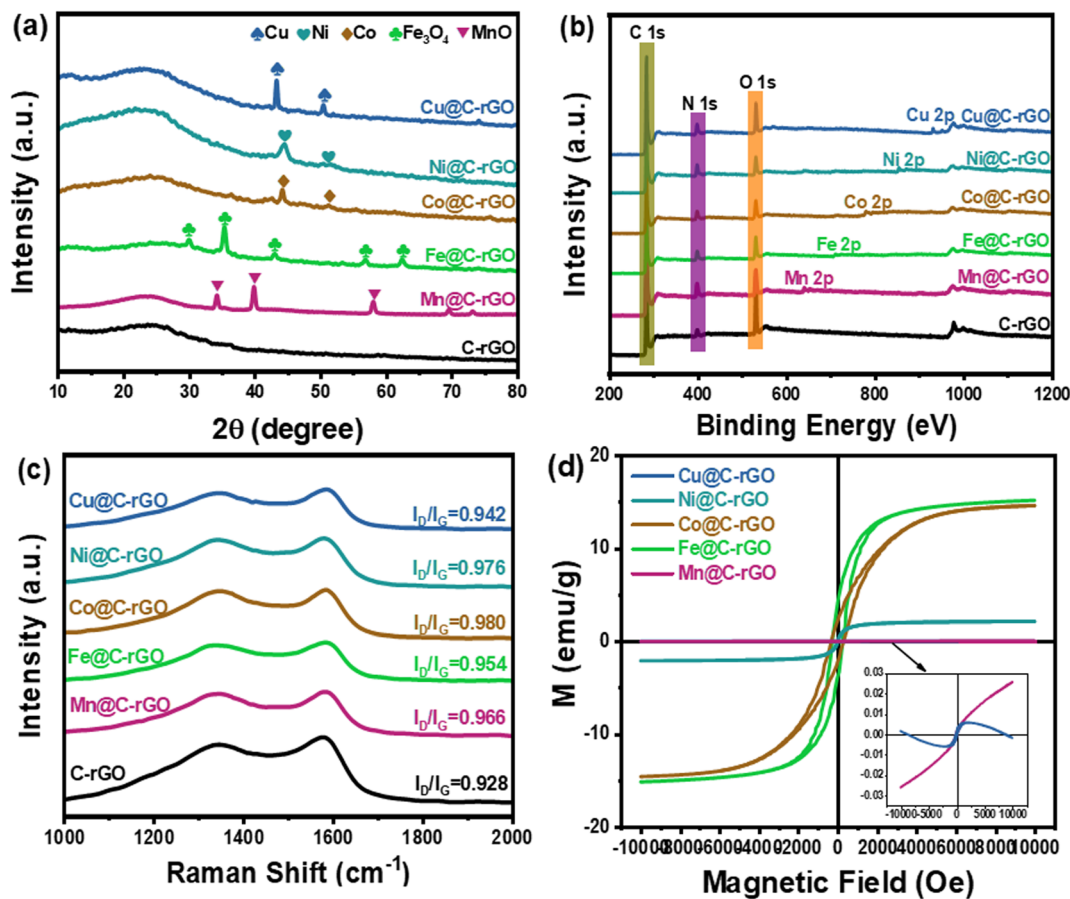
Fig. 2 Compositional characterization: (a) the XRD patterns, (b) XPS survey spectra, (c) Raman spectra and (d) the hysteresis loop of the samples.
