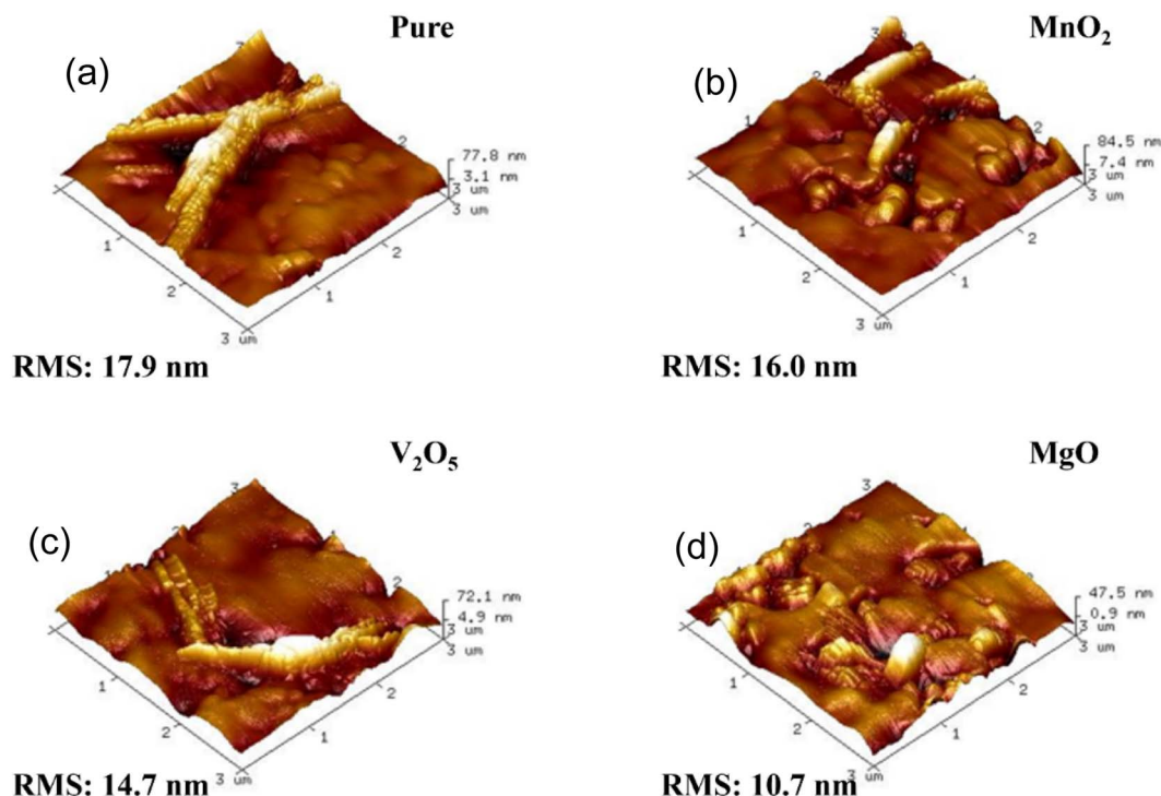
Fig. 10 AFM images of (a) pure PCBM and PCBM doped with (b) MnO 2 , (c) V 2 O 5 and (d) MgO.
