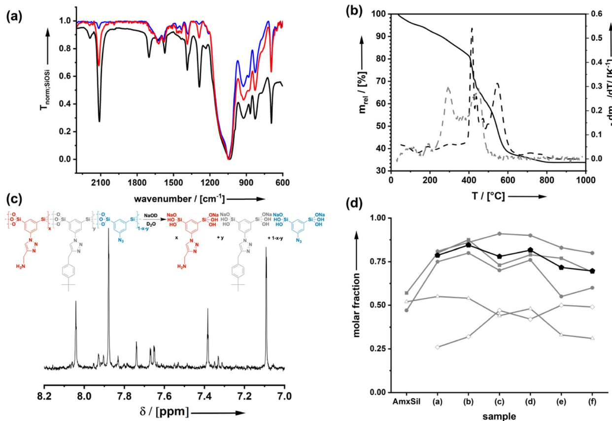
Fig. 1 (a) FT-IR spectra of AzSil (black), AmSil (red) and \text{Am}_x\text{Sp}_y(\text{d})\text{Sil} (blue; \text{R}_{\text{F}_2} = \text{tert-butyl phenyl} ). (b) TGA trace (solid line) for the oxidative decomposition of AmSp(d)Sil (black) and the first derivative (dashed line) in comparison to the decomposition steps of AmSil (grey). (c) ^1\text{H-NMR} spectrum (aromatic region) of the dissolved \text{Am}_x\text{Sp}_y(\text{d})\text{Sil} sample. (d) Results for the composition analysis of the different samples; squares ( x + y determined from IR), circles ( x + y determined from TGA), hashes ( x determined from NMR), triangles ( y determined from NMR), hexagons ( x + y determined from NMR), and pentagons ( x + y ; averaged value).
