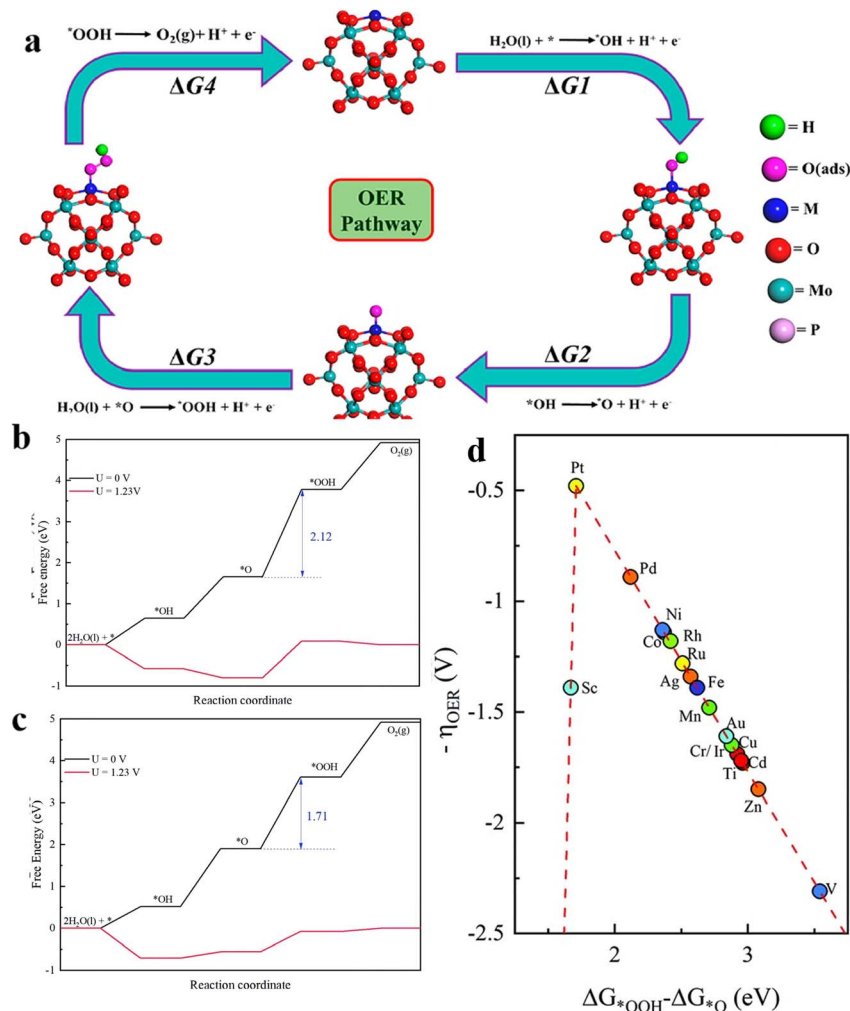
Fig. 5 (a) Schematic of the 4e⁻ OER pathway of the 4H site via the M₁/PMA cluster, reproduced with permission. 21 Copyright 2021, American Chemical Society. (b) Free energy diagrams of basic steps of the Pd@Sb monolayer and (c) Pd@Sb monolayer at different potentials. (d) The volcano curve between negative OER overpotential and \Delta G_{\text{OOH}^*} - \Delta G_{\text{O}^*} for TM@Sb monolayers. Reproduced with permission. 54 Copyright 2021, Royal Society of Chemistry.
