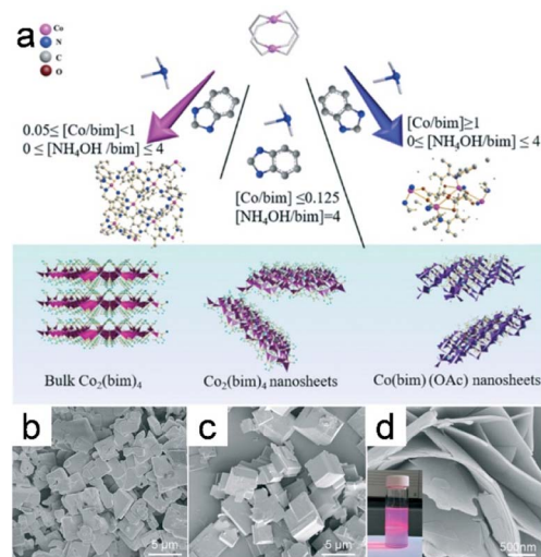
Fig. 8 (a) The diagram depicts the process for the synthesis of the Co 2 (bim) 4 , the UTCo 2 (bim) 4 , as well as the Co(bim)(OAc). SEM images of the Co 2 (bim) 4 prepared using varying amounts of NH 4 OH (Y value denotes the NH 4 OH/bim molar ratio): (b) Y = 0; (c) Y = 2; (d) Y = 4. (Panels a–d) Reproduced with permission. 19 Copyright 2019, Royal Society of Chemistry.
