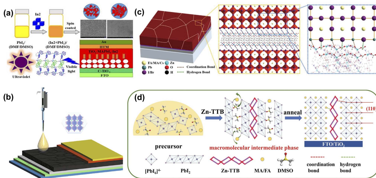
Fig. 7 (a) The design concept and device structure of [\text{In}_{0.5}\text{K}(3\text{-qlc})\text{Cl}_{1.5}(\text{H}_2\text{O})_{0.5}]_2\text{Zn} . Reproduced from ref. 43 with permission from Elsevier, copyright 2019. (b) The schematic diagram for fabricating n-i-p PSCs with the perovskite/In-BTC heterojunction as a light-harvesting layer. Reproduced from ref. 37 with permission from Springer Nature, copyright 2020. (c) Schematic illustration of the perovskite film with Zn-cbpp modification. Reproduced from ref. 44 with permission from Wiley-VCH, copyright 2021. (d) Schematic illustration of the Zn-TTB-regulated grain growth process by inducing a macromolecular intermediate phase. Reproduced from ref. 69 with permission from Wiley-VCH, copyright 2022.
