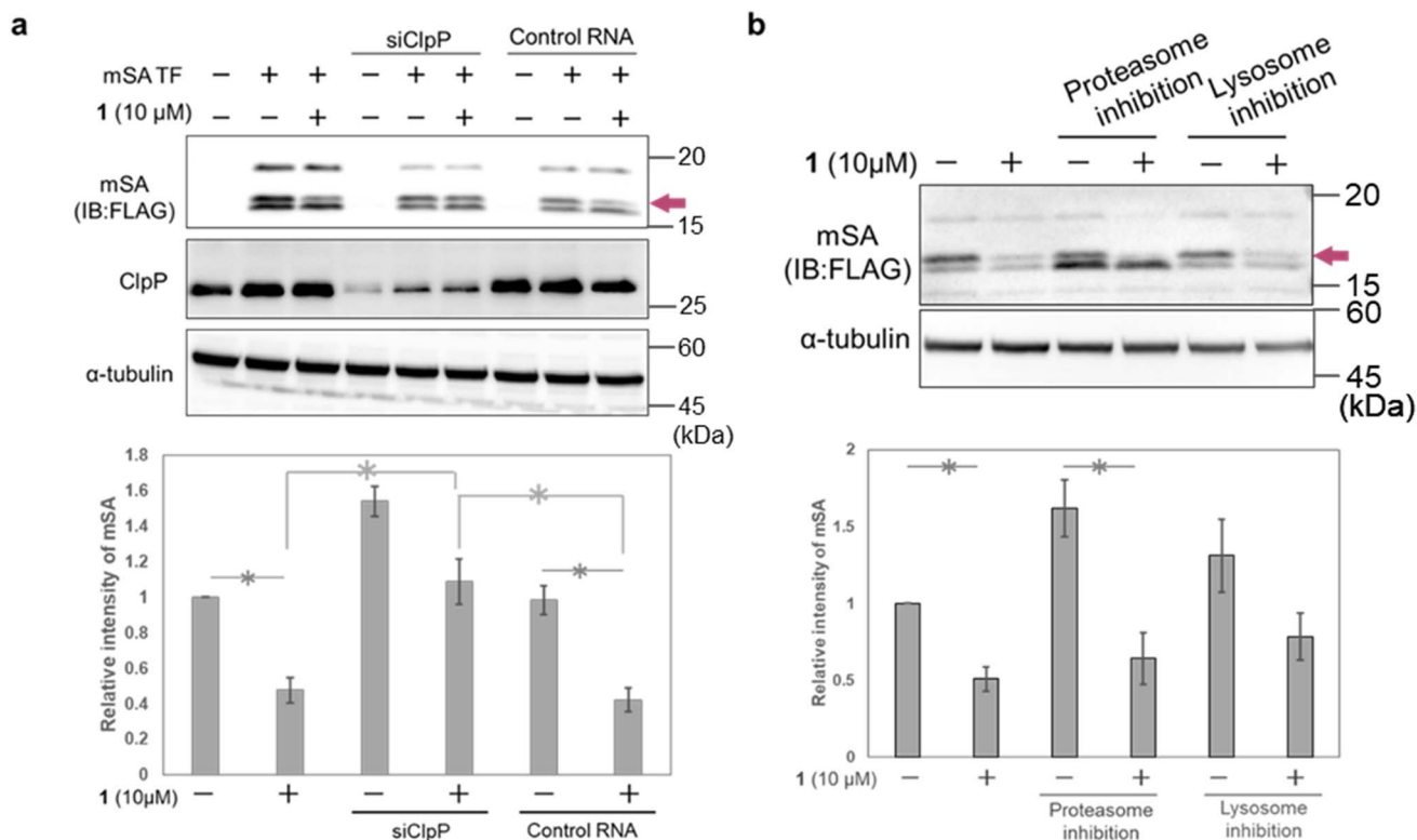
Fig. 5 Analyses of mSA degradation pathway. (a) Degradation of mSA induced by 48 h treatment with WY165 (1) in HeLa cells with ClpP knockdown by transfection of siClpP. TF stands for transfection. (b) Degradation of mSA induced by 48 h treatment with 1 in HeLa cells in the presence of an inhibitor of proteasome or lysosome. Proteasome inhibition was performed by treatment with 300 nM bortezomib. Lysosome inhibition was performed by co-treatment with 10 \mu M leupeptin and 30 mM \text{NH}_4\text{Cl} . Western blots and quantification results are shown. The data were normalized to the control value, taken as 1. Error bars indicate SEM ( n = 3 measurements). *: p < 0.05 , Student's t -test.
