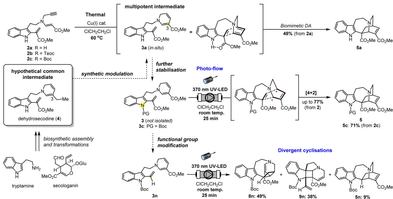
Fig. 7 Biosynthesis of dehydrosecodine (4) initiates from tryptamine and secologanin as building blocks. The thermal biomimetic [4 + 2] cycloaddition proceeds via a dehydrosecodine-type multipotent intermediate ( 3a → 5a ) facilitated by both heating and an intramolecular hydrogen-bonding. The new photo-flow approach features site-selective activation of DHP moiety using stabilised substrates 3 with indole N1 protection. A biradical reaction pathway enabled the divergent [4 + 2] and [2 + 2] cyclisations with minimal conformational changes in the pre-organised structures of 3c and 3n , respectively.
