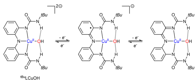
Scheme 9 Characterized oxidation states reached via reduction/oxidation of t Bu 4 LCuOH. Adapted from ref. 73.
