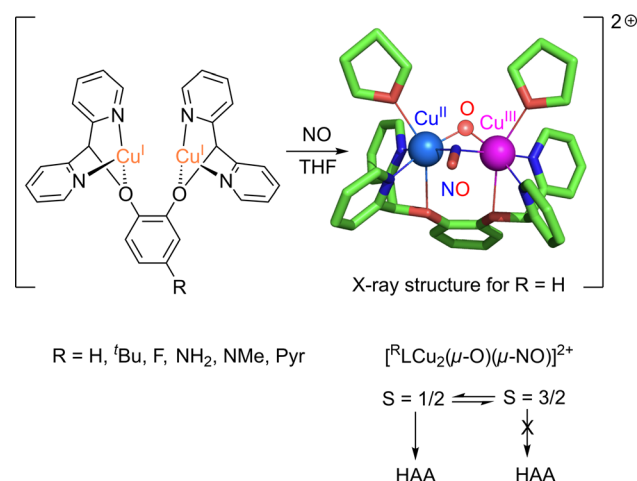
Fig. 10 Synthesis of [R L Cu 2 (μ-O)(μ-NO)] 2+ species and influence of the spin state on HAA reactivity from ref. 73 and 74.
