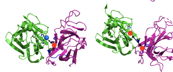
Fig. 2 Uncoupled binuclear copper-containing monooxygenases, PHM and D \beta H. (a) and (b) reactions catalyzed by PHM and D \beta H, respectively; (c) X-ray structure of PHM from Rattus norvegicus showing the two domains (Cu M domain in green and Cu H domain in magenta) connected by a loop (in blue) in which each domain binds a single copper atom spaced from each other by approximately 11 Å and (d) structure of the Cu M -superoxido intermediate in PHM (PDB ID 1opm); (e) and (f) X-ray structure of the human D \beta H (PDB ID 4zel) showing the open (e) and the closed (f) forms. Only the Cu M domain of the closed form contains a copper atom, the other copper ions (red sphere) are manually placed.
