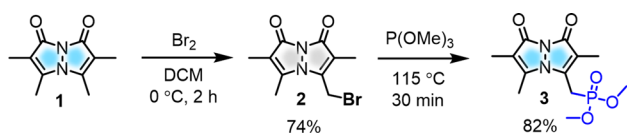
Scheme 1 Synthesis of key bimane precursor.
