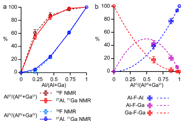
Fig. 4 (a) Plots of the fraction of octahedral sites occupied by Al, \text{Al}^{\text{VI}} ( \text{Al}^{\text{VI}}/(\text{Al}^{\text{VI}} + \text{Ga}^{\text{VI}}) ), in red, and of tetrahedral sites occupied by Al, \text{Al}^{\text{IV}} ( \text{Al}^{\text{IV}}/(\text{Al}^{\text{IV}} + \text{Ga}^{\text{IV}}) ), in blue, as a function of composition for (\text{Al}_x\text{Ga}_{1-x})_3\text{P}_3\text{O}_{12}\cdot\text{F}\cdot\text{mim} , determined from a combination of ^{27}\text{Al} and ^{71}\text{Ga} NMR spectroscopy (solid lines) and from ^{19}\text{F} NMR spectroscopy (dashed lines). (b) Plots of expected relative intensities of the Al-F-Al, Al-F-Ga and Ga-F-Ga signals against octahedral site occupancy, assuming a random distribution of the cations (dashed lines) and their experimental intensities (circles). In both parts error bars indicate estimated uncertainties in the ^{71}\text{Ga} and ^{19}\text{F} spectral integrals.
