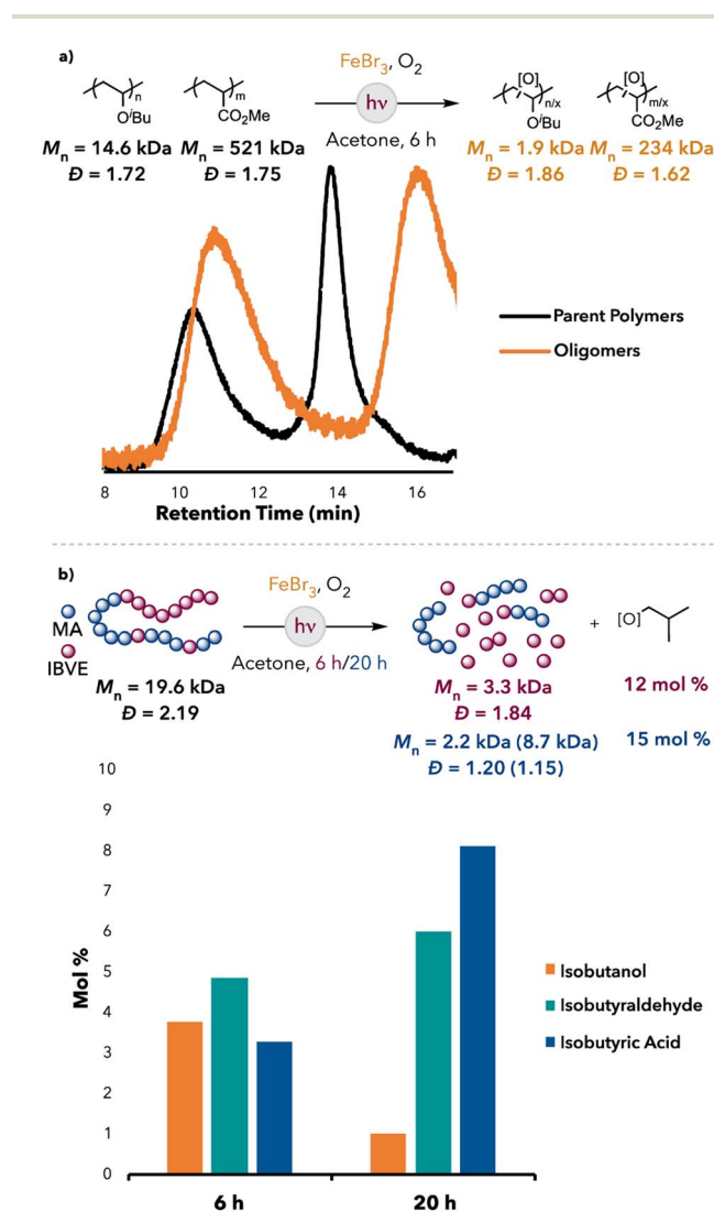
Fig. 5 (a) PIBVE and PMA mixture degradation with FeBr 3 . (b) Poly(-IBVE-co-MA) degradation results: Lower M_n peak (higher M_n peak).
