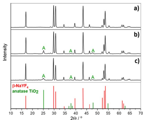
Fig. 2 XRD patterns of (a) UCPs ( \beta\text{-NaYF}_4\text{:Yb}^{3+},\text{Tm}^{3+} ) crystals, (b) UCPs + P25 ( \beta\text{-NaYF}_4\text{:Yb}^{3+},\text{Tm}^{3+} mixed with P25) sample and (c) UCPs@ \text{TiO}_2 ( \beta\text{-NaYF}_4\text{:Yb}^{3+},\text{Tm}^{3+} coated with \text{TiO}_2 ) sample. "A" indicates reflections characteristic for \text{TiO}_2 anatase.
