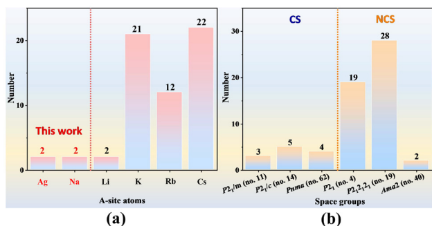
Fig. 2 Statistical analyses showing the different A-site atoms (a) and space groups (b) in the A^I\text{RE}^{\text{III}}\text{C}^{\text{IV}}\text{Q}^{\text{VI}} ( A^I = \text{Ag, Li-Cs; RE}^{\text{III}} = \text{Y, La-Nd, Sm-Yb; C}^{\text{IV}} = \text{Si, Ge; Q}^{\text{VI}} = \text{S, Se} ) family compounds.
